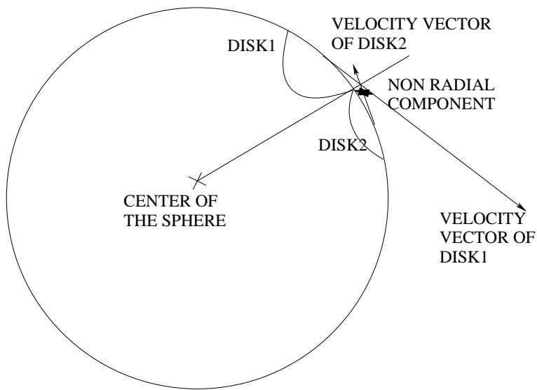
Figure 4: Schematic representation of the non radial component of the relative velocity vector after an interaction between two disks on the sphere
