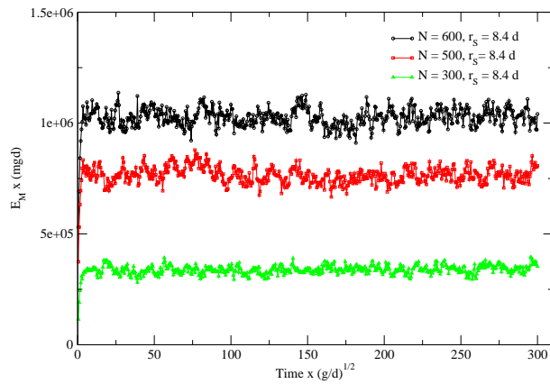
Figure 3: Total kinetic energy as a function of time for a constant sphere radius (in unit of disk diameter) but different number of disks
