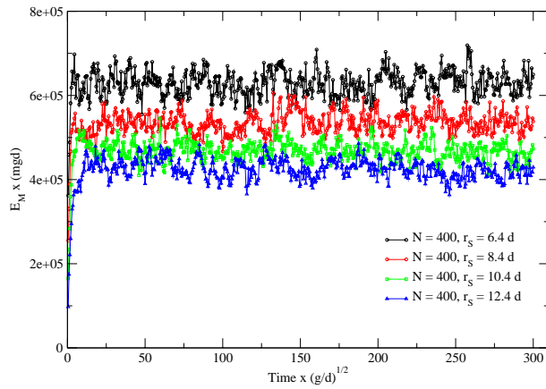
Figure 2: Total kinetic energy as a function of time for the different sphere radii (in unit of disk diameter) but a constant number of disks
